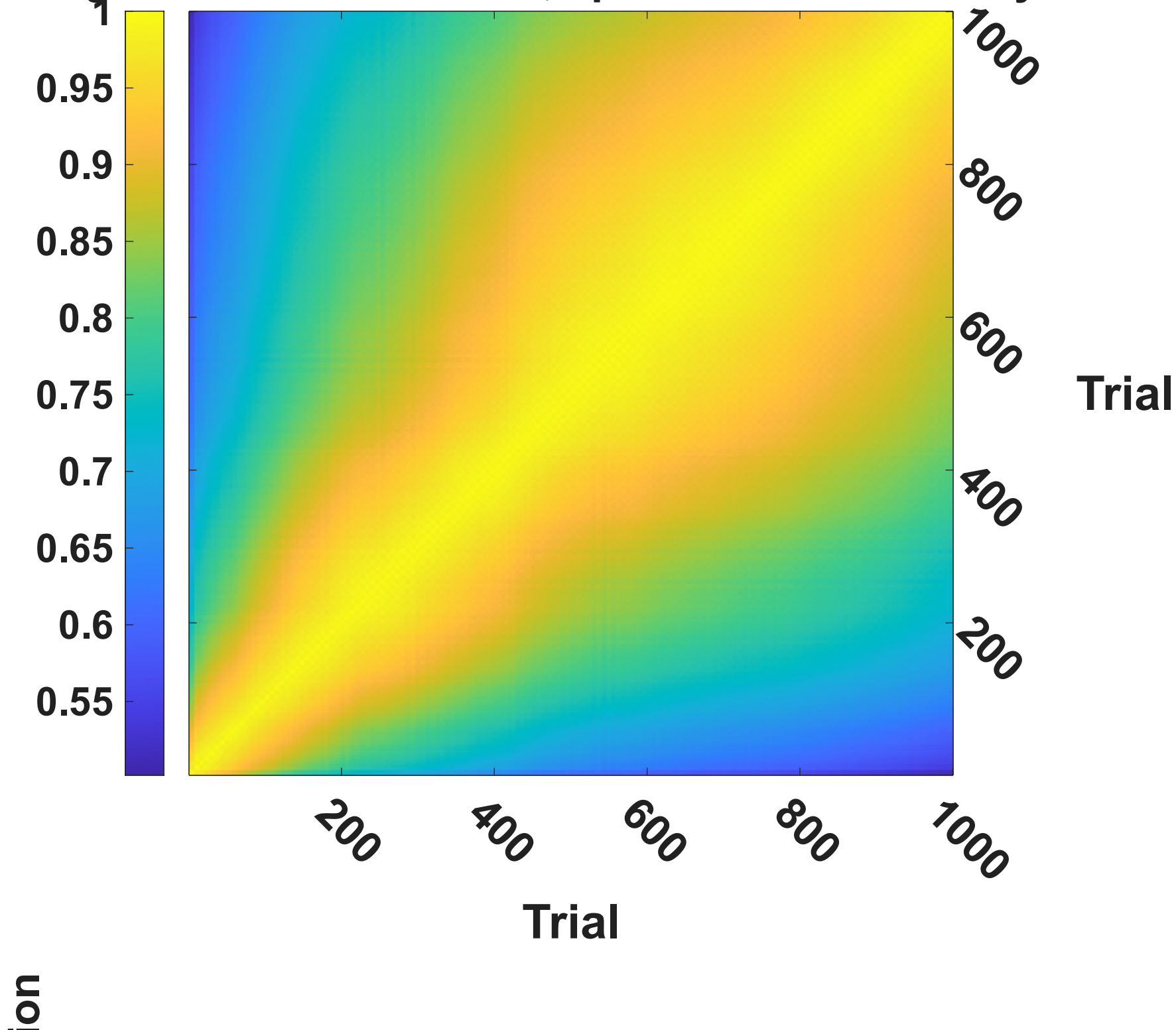
Averaged on 10 Simulations, spike counts Similarity Matrix
